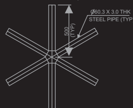
6-Way Bracket Details
